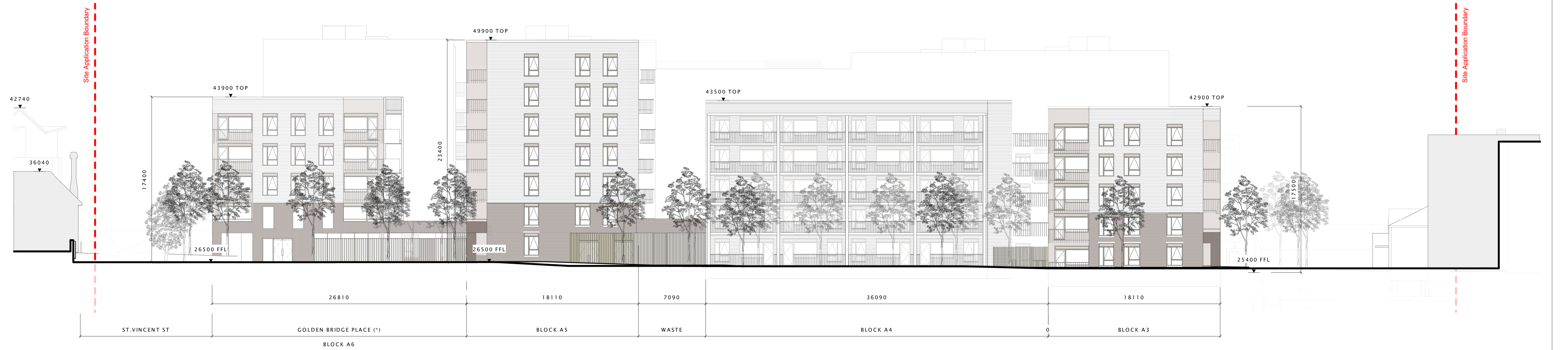
2 CONTEXTUAL ELEVATION - S 1 : 200
